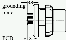
Figure 2: Grounding Plate and PCB Pin Length of ZK Receptacle
