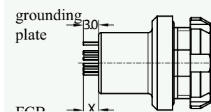
Figure 1: Grounding Plate and PCB Contact Length of Z8 Receptacle
