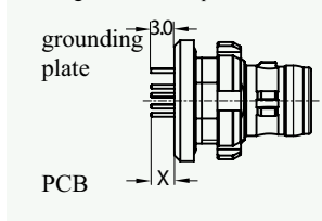
Figure 3: Grounding pin and PCB Pin Length of ZW Receptacle
