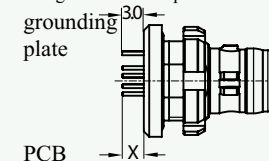
Figure 3: Grounding pin and PCB Pin Length of ZW Receptacle
