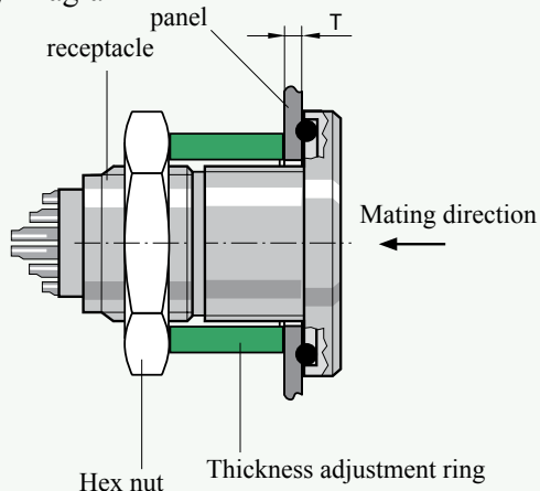
Assembly Diagram
